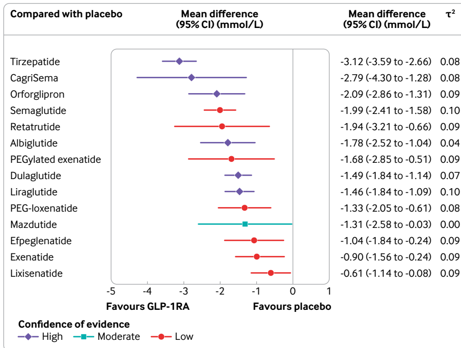
Fig 5 | Forest plot of network effect sizes between GLP-1RAs and placebo for fasting blood glucose. Certainty of evidence is visually represented in the forest map, with varying colours indicating different confidence levels. The complete CINeMA assessments are shown in appendix 9. GLP-1RA=glucagon-like peptide-1 receptor agonist; PEG-loxenate=polyethylene glycol loxenate
